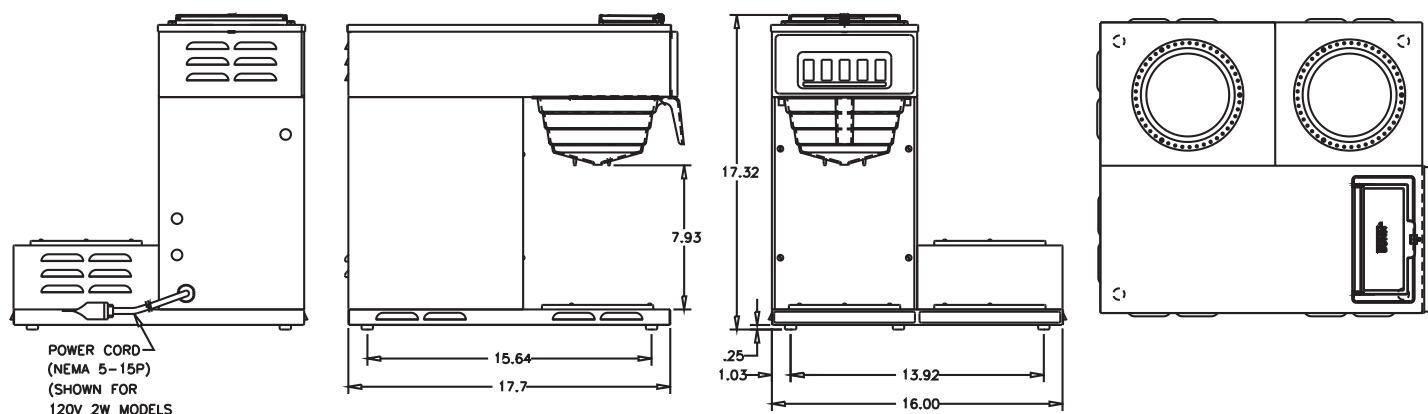
3 Lower Warmers
